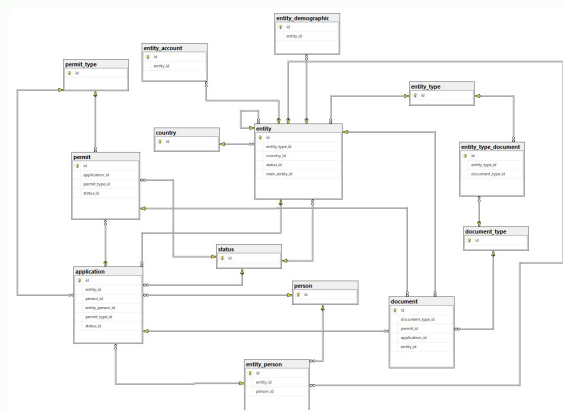
The ERaAS entity relationship model
